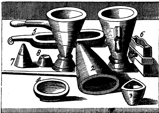
Fig. 121. 1. "The form of the common cup cast in brass. 2. A cup made of smith's work [to receive the melted antimony and gold]. 3. A crucible for the work [ i.e. , the casting the antimony and gold]. 4. A flat test [cupel] for it. 5. The ingot [mould]. 6. The plates [mould]. 7. The cast antimony with a gold regulus. 8. The cast antimony when the gold regulus is beaten from it." (Pettus.)
